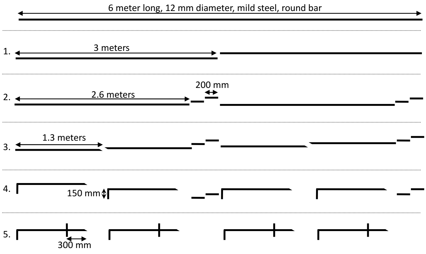
Figure 10. Diagram of the production of custom metal floating crop cover stakes. Numbers refer to the above instructions.
